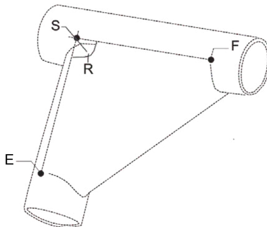
Drawing.8.6 Gusset
